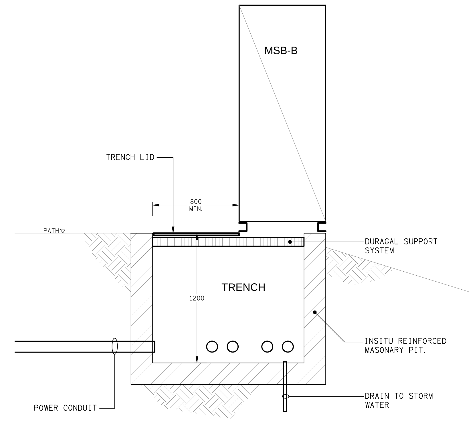
DETAIL B MSB-B & TRENCH SECTION SCALE 1: 20
