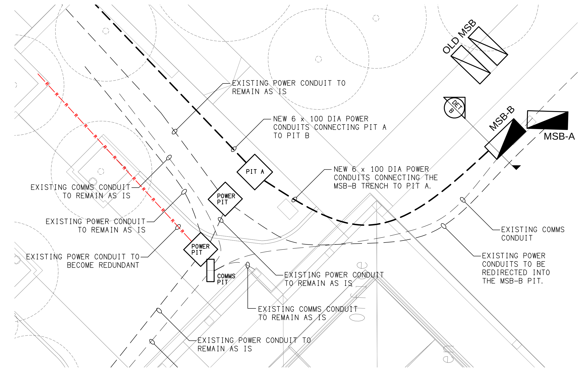
DETAIL A MSB & PIT PLAN SCALE 1: 100
